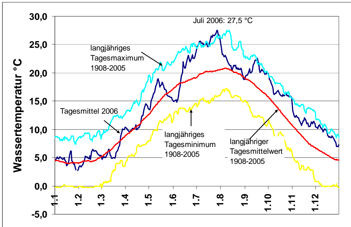
River Rhine water temperatures in 2006 at Lobith compared with long-term values
